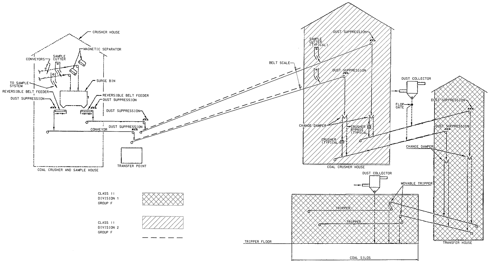
FIGURE 1 PROCESS FLOW DIAGRAM COAL HANDLING SYSTEM
